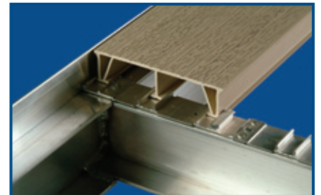
Cut-a-way showing frame and how vinyl decking is attached
