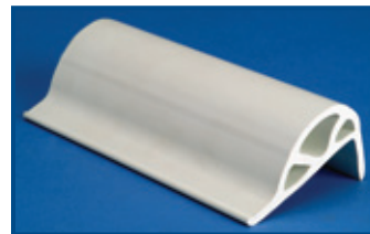
"L" Vinyl Rub Rail Wraps from side to top of aluminum frame.
